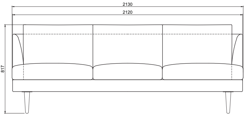
3-SEATER SOFA
