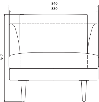
LOUNGE CHAIR
