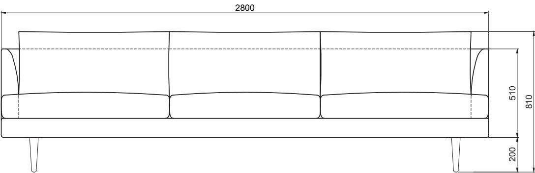
4-SEATER SOFA
