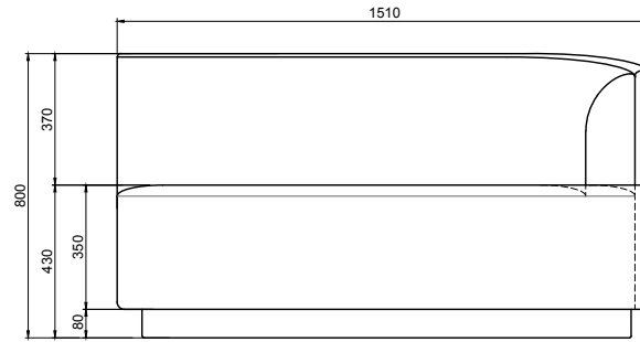
2-SEATER MODULE, RIGHT
